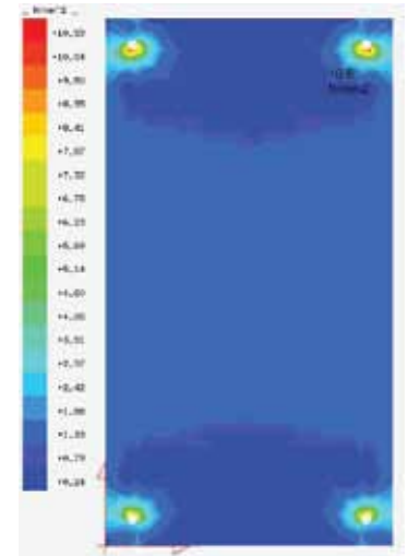
The glass unitary efforts diagram.
