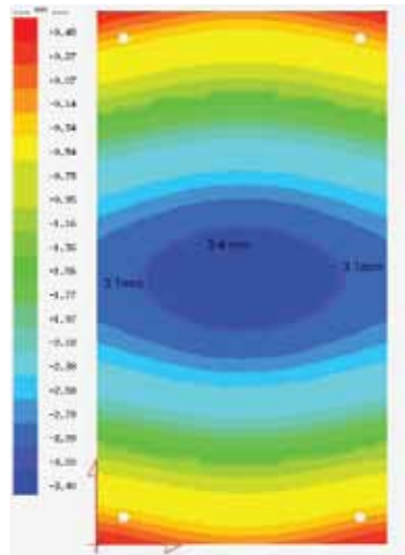
The glass strains diagram.
